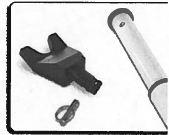
A removable pin releases the yoke end for sliding door applications.
